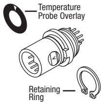
TEMP PROBE CONNECTOR RPI Part #GEC008 OEM Part #300681
