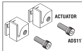
AUTO RECLINE ACTUATOR RPI Part #PCA747 OEM Part #007660
