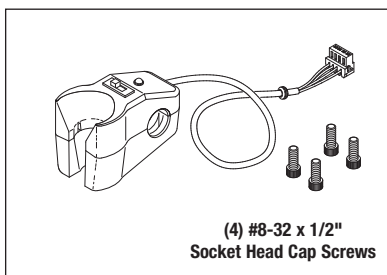
(4) #8-32 x 1/2" Socket Head Cap Screws
