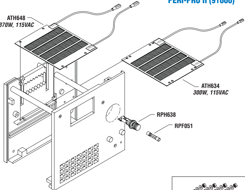
Mounting Hardware included with Heating Elements (RPI Part #ATH634 & ATH648)
